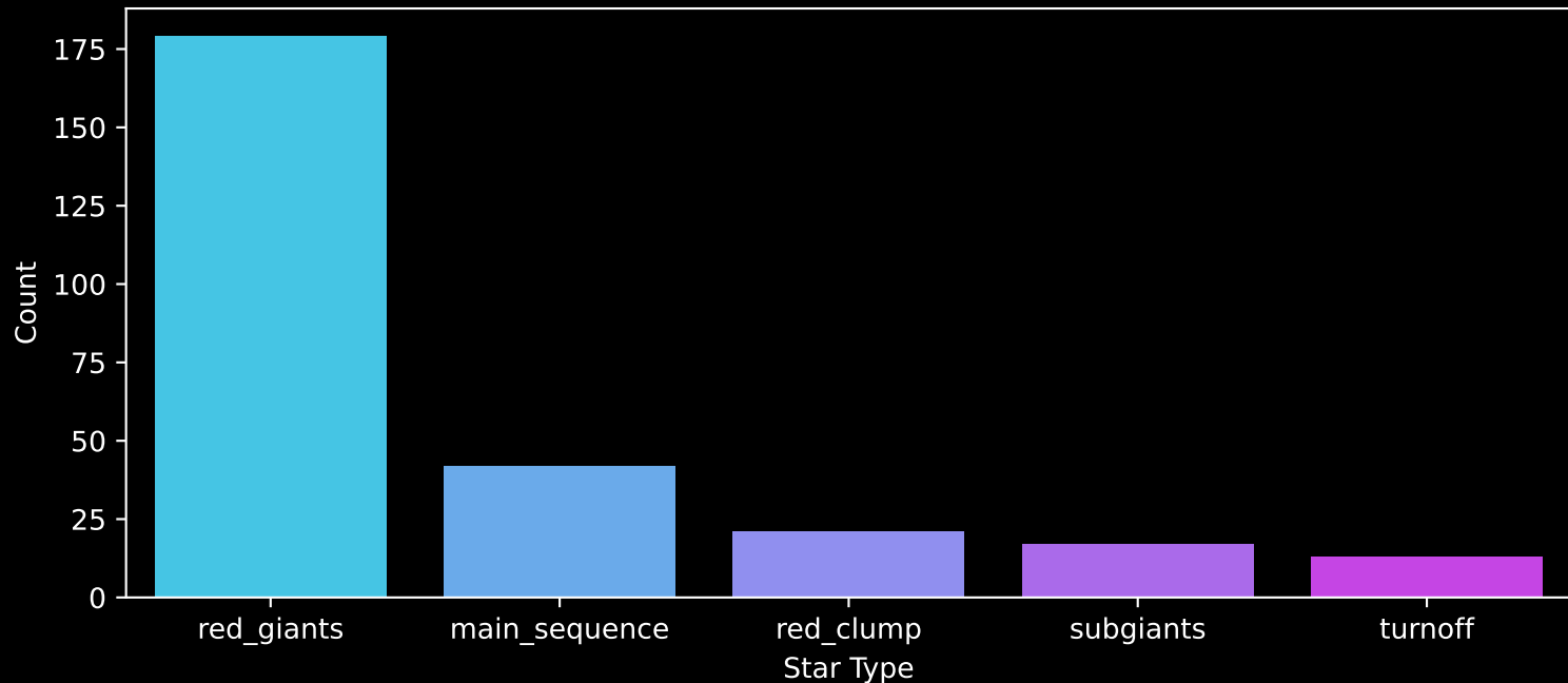
APOGEE DR17 Field: [311+00] Count plot of Star Type
