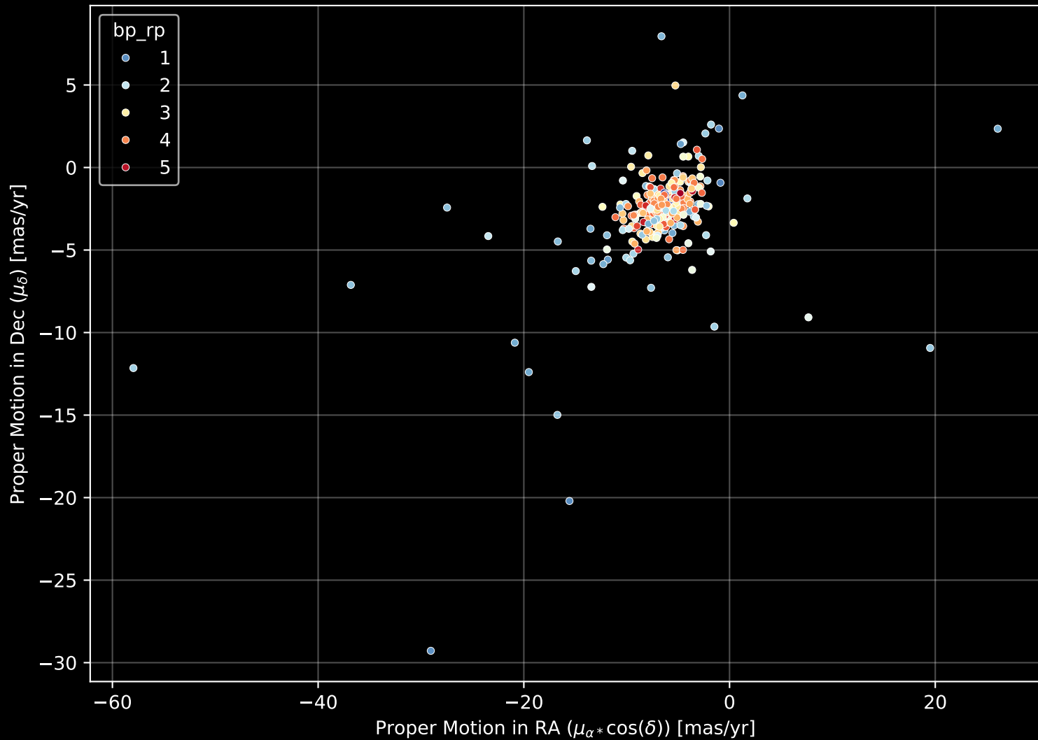
APOGEE DR17 Field: [311+00] Proper Motion Diagram (n= 272)
