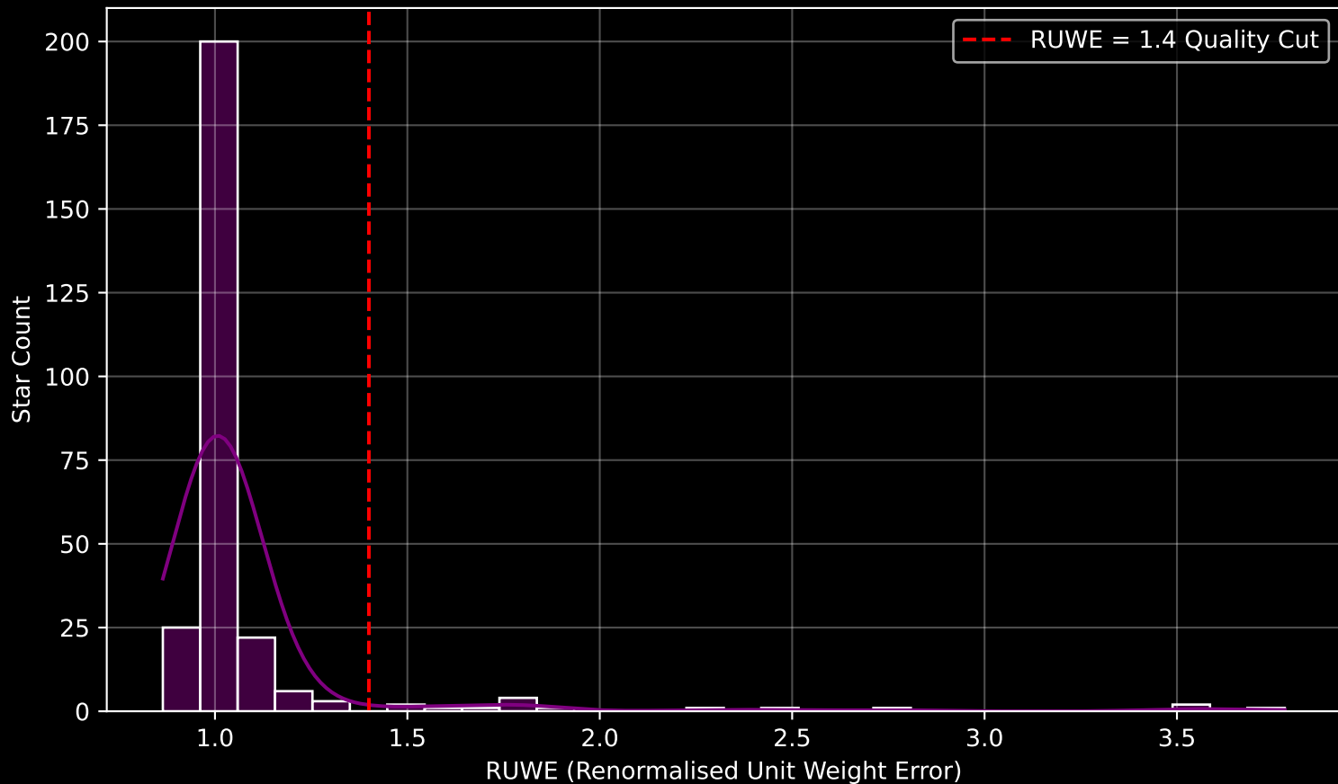
GAPOGEE DR17 Field [311+00] RUWE Distribution (n= 271)
