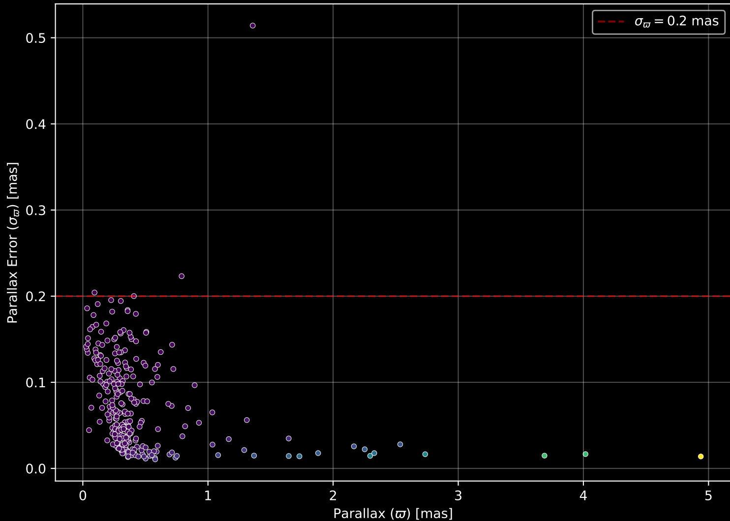
APOGEE DR17 Field: [311+00] Parallax Quality (n= 272)
