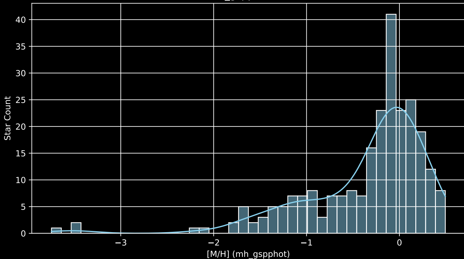
APOGEE DR17 Field: [311+00 [M/H] (mh_gspphot) (n= 248)
